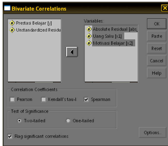
Correlations
